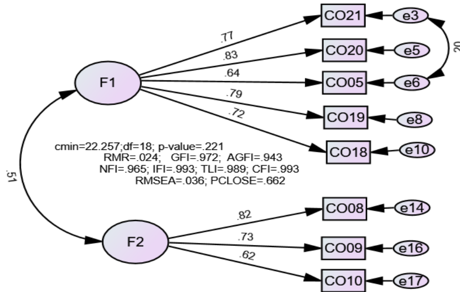
Figure 3. Standardised solution of the measurement model: Budget overrun.
