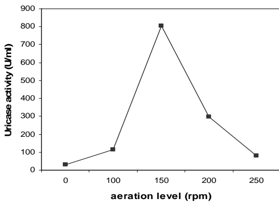
Figure 3: Effect of different aeration levels on uricase enzyme production
