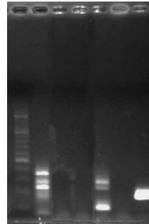
FIGURE 11 Ethidium bromide- stained agarose gel (1% w/v) displaying PCR product of DNA extracted from laboratory strains using designed PCR primer nahA4 .
