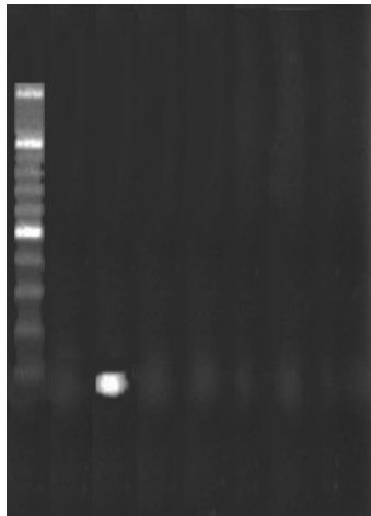
FIGURE 9 Ethidium bromide-stained agarose gel (1% w/v) of amplified PCR product of DNA extracted from laboratory strains using nahA2 primer set.
