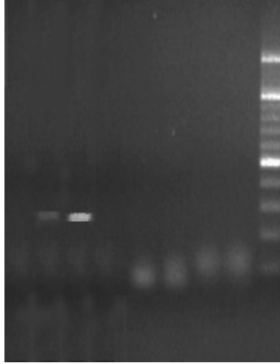
FIGURE 8 Ethidium bromide-stained agarose gel (1% w/v) of PCR product of DNA extracted from laboratory bacterial strains collection amplified using nahA1 primer set.
