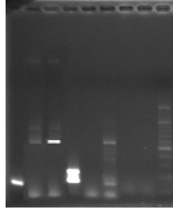
FIGURE 10 Ethidium bromide-stained agarose gel (1% w/v) displaying amplified PCR product using designed PCR primer nahA3 .
